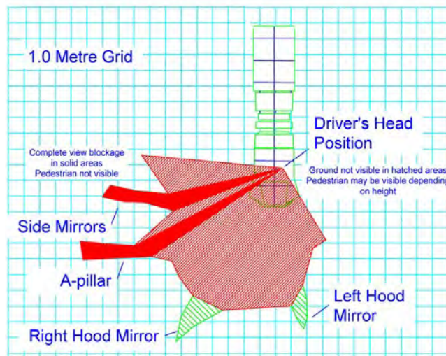
Field of View - Blind Spot Areas from a Heavy Vehicle
